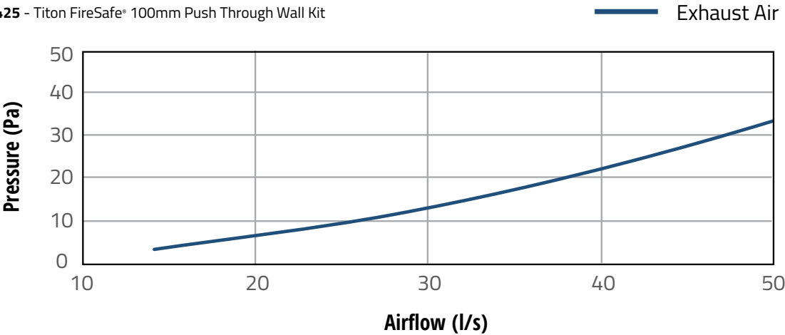
TA425 - Titon FireSafe® 100mm Push Through Wall Kit
